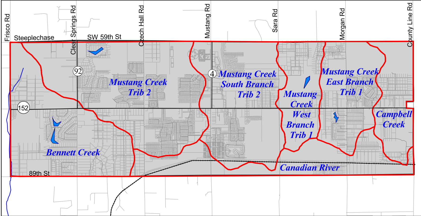
Figure 2-2 City of Mustang Drainage Basins
